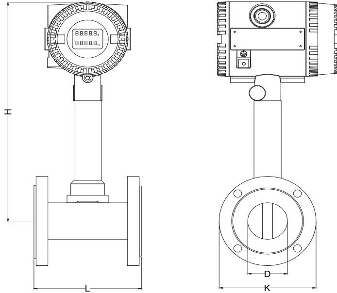
Dimension for ANSI CL150 Flanged
