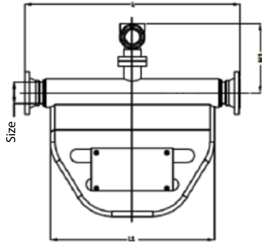
Micro-bend Shaped Sensor (Size ½" to 8")
