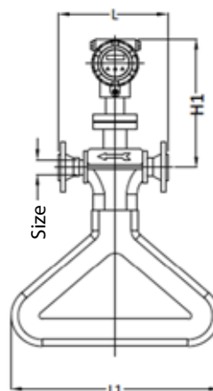
Triangle Shaped Sensor (Size ½" to 1")
